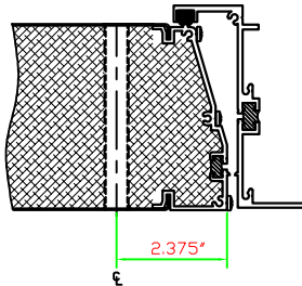
4" DOOR 1 GASKET
