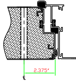
4" DOOR 2 GASKET
