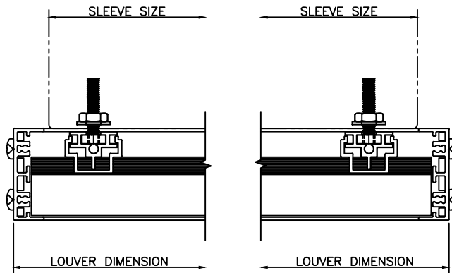
3 LOUVER JAMB HANG ON - MINIMUM WIDTH
