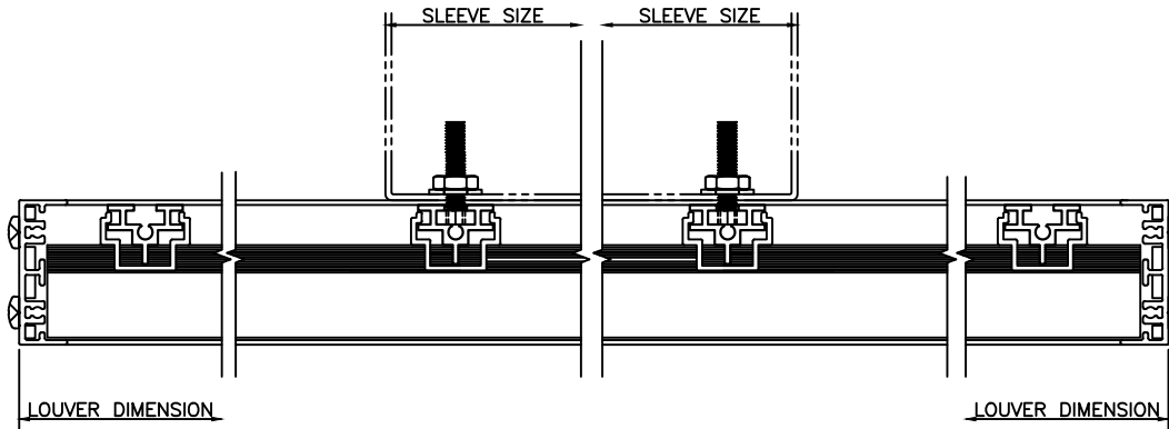
5 LOUVER JAMB HANG ON - LOUVER PAST OPENING
