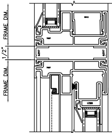
13 MULL STRIP SERIES 70 FIXED/SASH
