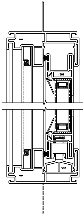
1 SASH HEAD SERIES 70 SLIDER
