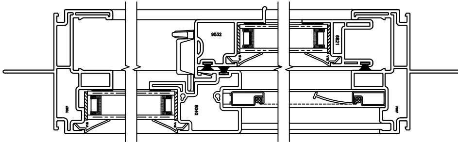
8 SASH JAMB SERIES 70 SLIDER
