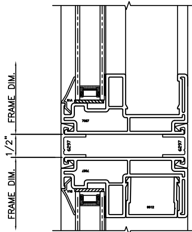
12 MULL STRIP SERIES 70 FIXED/FIXED
