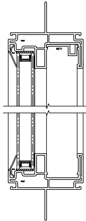
SERIES 70 SLIDER
