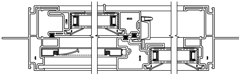
5 SASH JAMB SERIES 70 SLIDER
