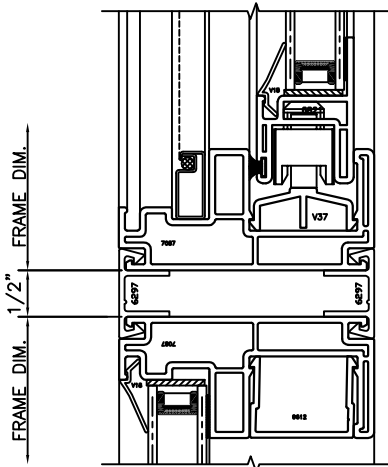
11 MULL STRIP SERIES 70 SASH/FIXED
