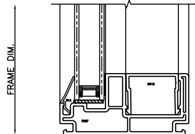
12 SILL SERIES 70 FIXED
