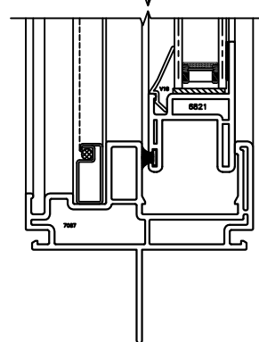
9 MULL STRIP SERIES 70 SH-SH
