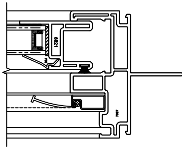
7 SASH JAMB SERIES 70 HUNG
