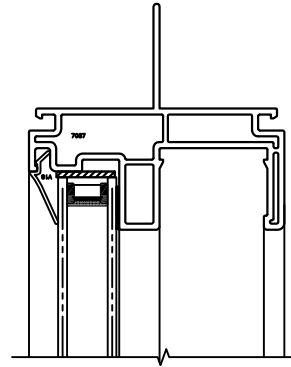
1 FIXED HEAD SERIES 70 HUNG
