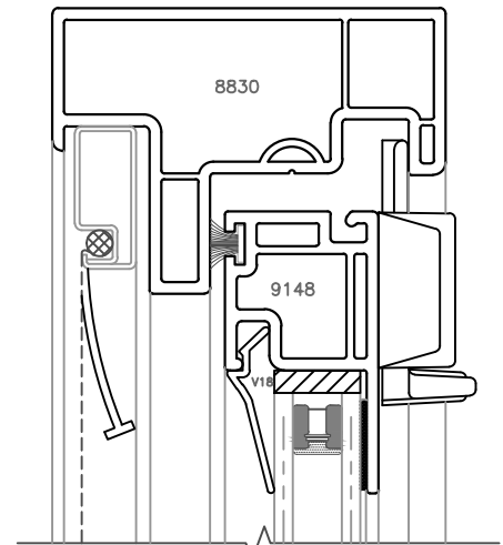
1 HEAD SERIES 70 V200 PI HOPPER
