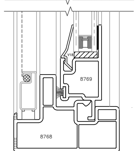
2 SILL SERIES 70 V200 PI HOPPER
