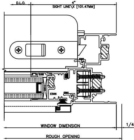
81 RIGHT JAMB LOWER 3270 DOUBLE HUNG
