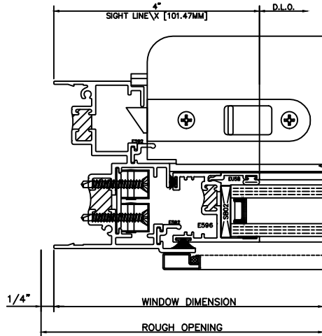
80 LEFT JAMB LOWER 3270 DOUBLE HUNG
