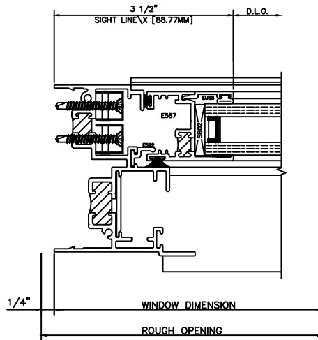
80 LEFT JAMB LOWER 3270 DOUBLE HUNG
