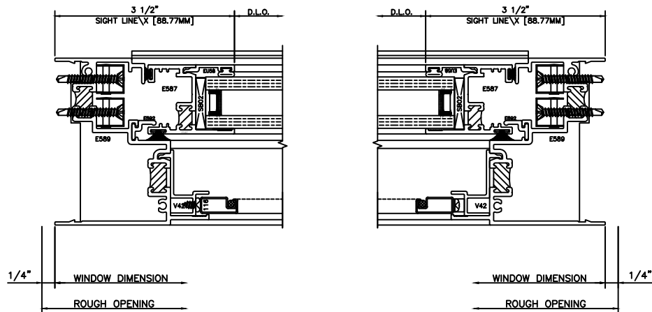
67 LEFT JAMB LOWER 3260 SINGLE HUNG
