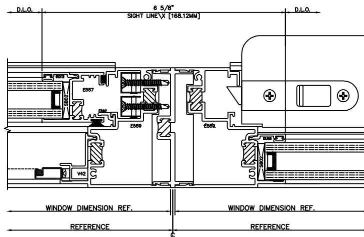
69 IMPOST 3260 SINGLE HUNG
