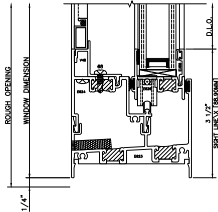
44 SASH SILL 3210 SLIDER-7LB SILL
