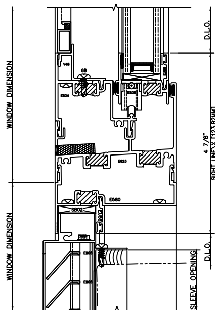
56 SASH SILL 3210 SLIDER-7LB SILL 3250 FRONT SET PTAC LOUVER
