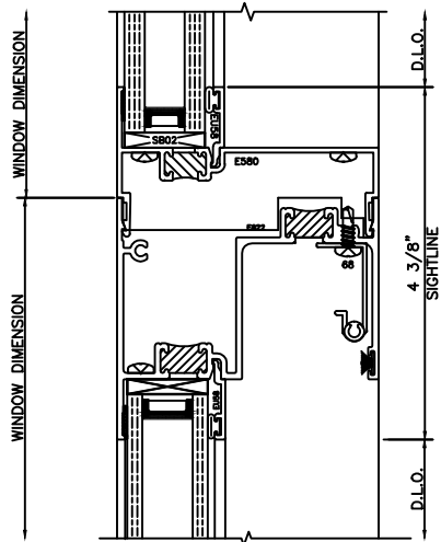
57 STACK 3250 FRONT SET FIXED 3210 SLIDER FIXED HEAD
