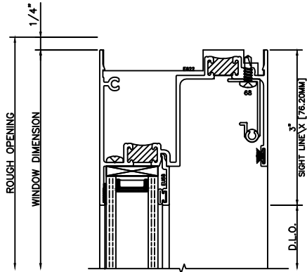
41 FIXED HEAD 3210 SLIDER
