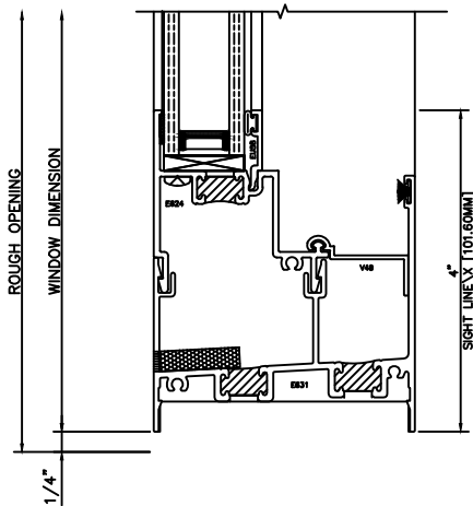
45 FIXED SILL 3210 SLIDER-10 LB SILL
