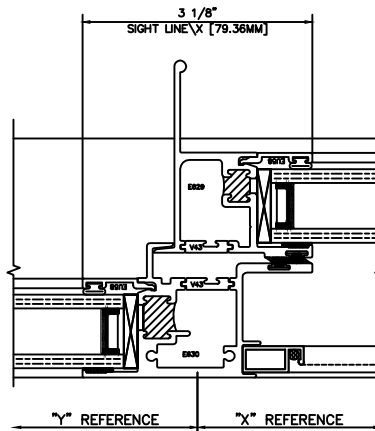
54 MTG RAIL 3210 SLIDER OXOL
