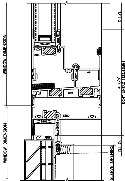
59 FIXED SILL 3210 SLIDER-7LB SILL 3250 FRONT SET PTAC LOUVER
