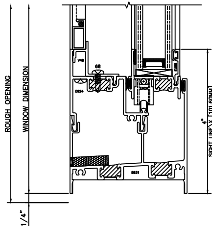
46 SASH SILL 3210 SLIDER-10 LB SILL
