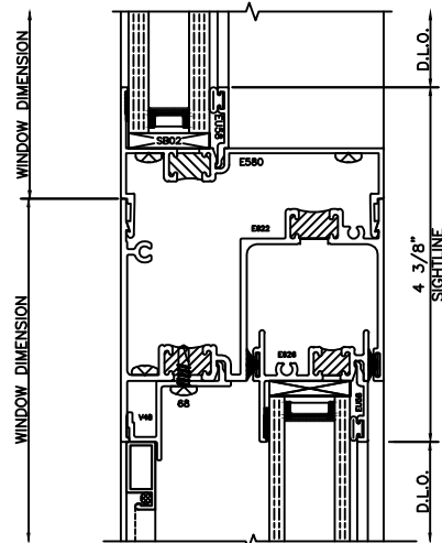
58 STACK 3250 FRONT SET FIXED 3210 SLIDER SASH HEAD
