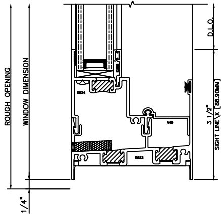
42 FIXED SILL 3210 SLIDER-7LB SILL
