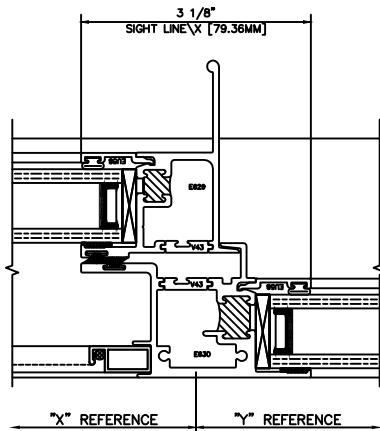
53 MTG RAIL 3210 SLIDER OXOR
