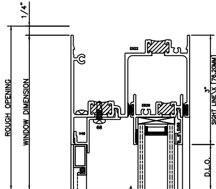
43 SASH HEAD 3210 SLIDER
