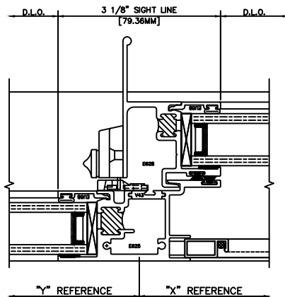
51 MTG RAIL 3210 SLIDER XO
