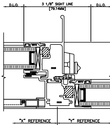
48 MTG RAIL 3210 SLIDER OX
