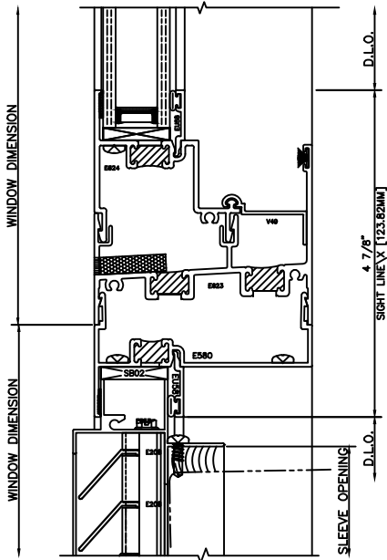
55 FIXED SILL 3210 SLIDER-7LB SILL 3250 FRONT SET PTAC LOUVER
