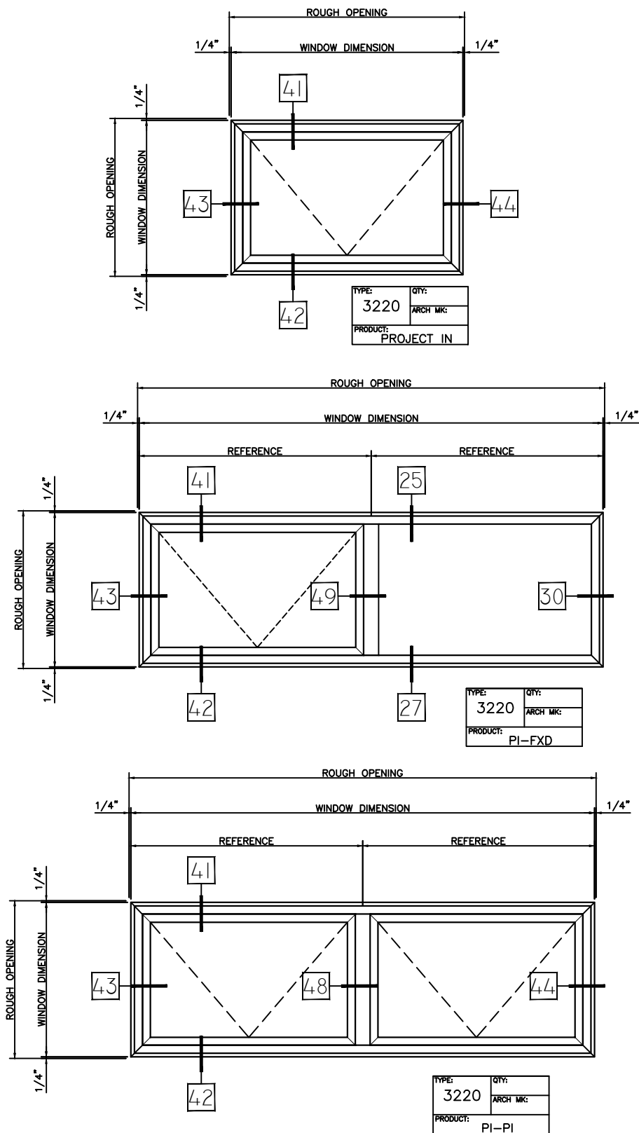
HALF SCALE DETAILS
