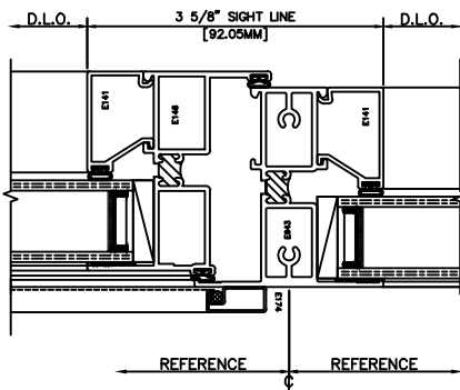
49 VERTICAL MUNTIN 3220 PROJECT IN-FIXED
