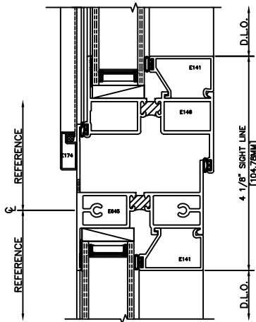
45 MTG RAIL 3220 PROJECT IN/FIXED
