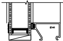
G6 1" INSUL. UNIT 1/8" - 3/4" A.S. - 1/8"
