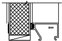
P1 1" NOM. INSUL. PANEL TYPICAL 3 PLY STYLE MAKE UP TO BE SPECIFIED
