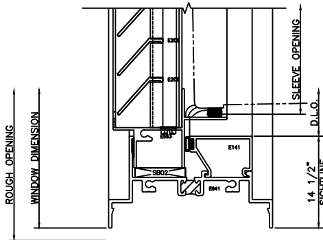
34 SILL @ LOUVER 3220 CENTER SET
