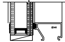
L2 1" INSUL. UNIT 3/16"-1/2" A.S.-1/4" LAMI- (1/8"-030 INNERLAYER-1/8")
