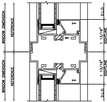
32 STACK 3220 CENTER SET
