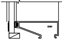
G1 1/4" NOM. GLAZING
