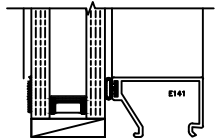
G4 1" INSUL. UNIT 1/4" - 1/2" A.S. - 1/4"
