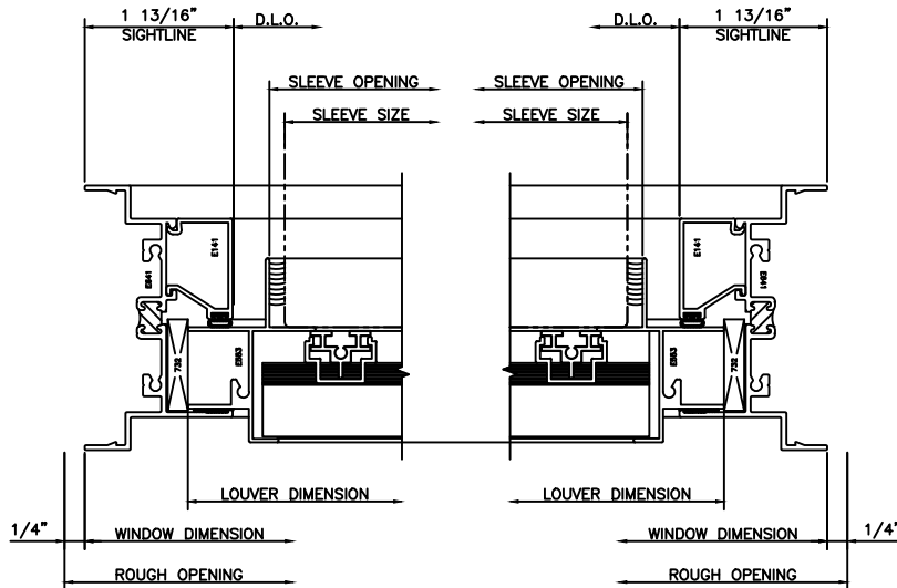
39 LOUVER JAMB @ SLEEVE OPENING 3220 CENTER SET
