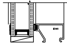
G5 1" INSUL. UNIT 3/16" - 5/8" A.S. - 3/16"
