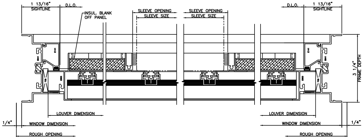
35 LOUVER JAMB @ BLANK OUT 3220 CENTER SET
