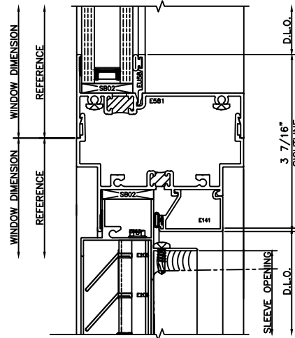
33 STACK @ LOUVER 3220 CENTER SET
