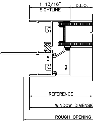
11 FIXED JAMB OUTSIDE GLAZED
