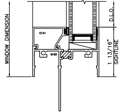
10 FIXED SILL AT O.G. PANEL
