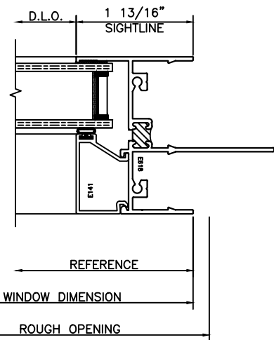
13 FIXED JAMB OUTSIDE GLAZED
