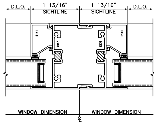
7 FIXED STACK VERTICAL STACKING JAMB
