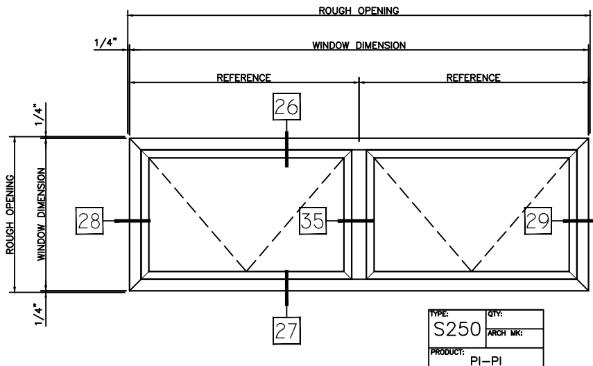
HALF SCALE DETAILS
