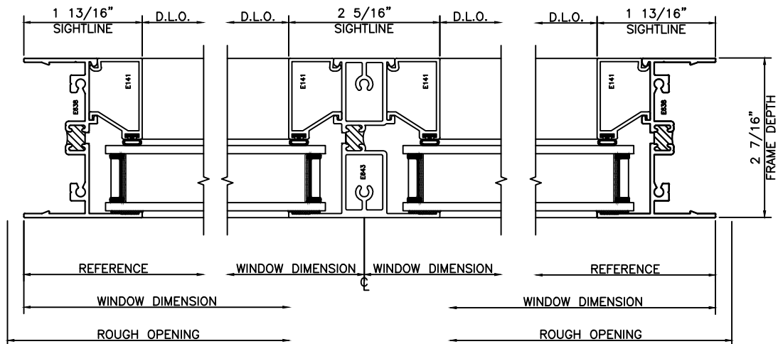
HALF SCALE DETAILS
