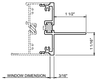
E759 THERMALLY BROKEN ALUMINUM NAIL FIN
