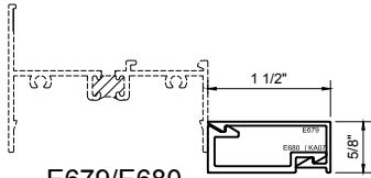
E679/E680 1 1/2" X 5/8" INTERIOR BOX TRIM.
