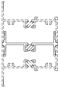
E527 TRANSITIONAL EXPANSION STACK MULL
