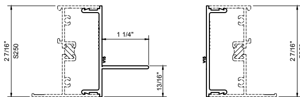
V15 FRAME FILLER WITH AND W/O FIN VINYL
