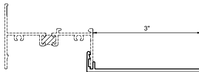
E526 FRAME ANCHOR
