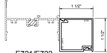
E721/E722 1 1/2" X 1 1/2" INTERIOR BOX TRIM.
