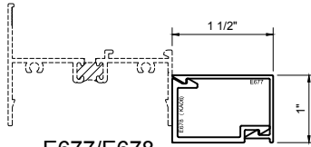
E677/E678 1 1/2" X 1" INTERIOR BOX TRIM.
